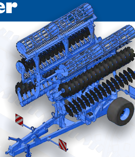
Transport position
